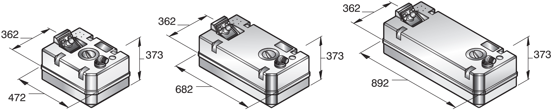
Vuilwater tanks / Waste water tanks
